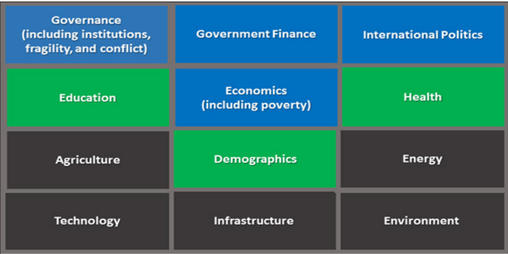
Figure 1: Models Within the IFs Forecasting System. Source: (Hughes and Hillebrand 2008).
