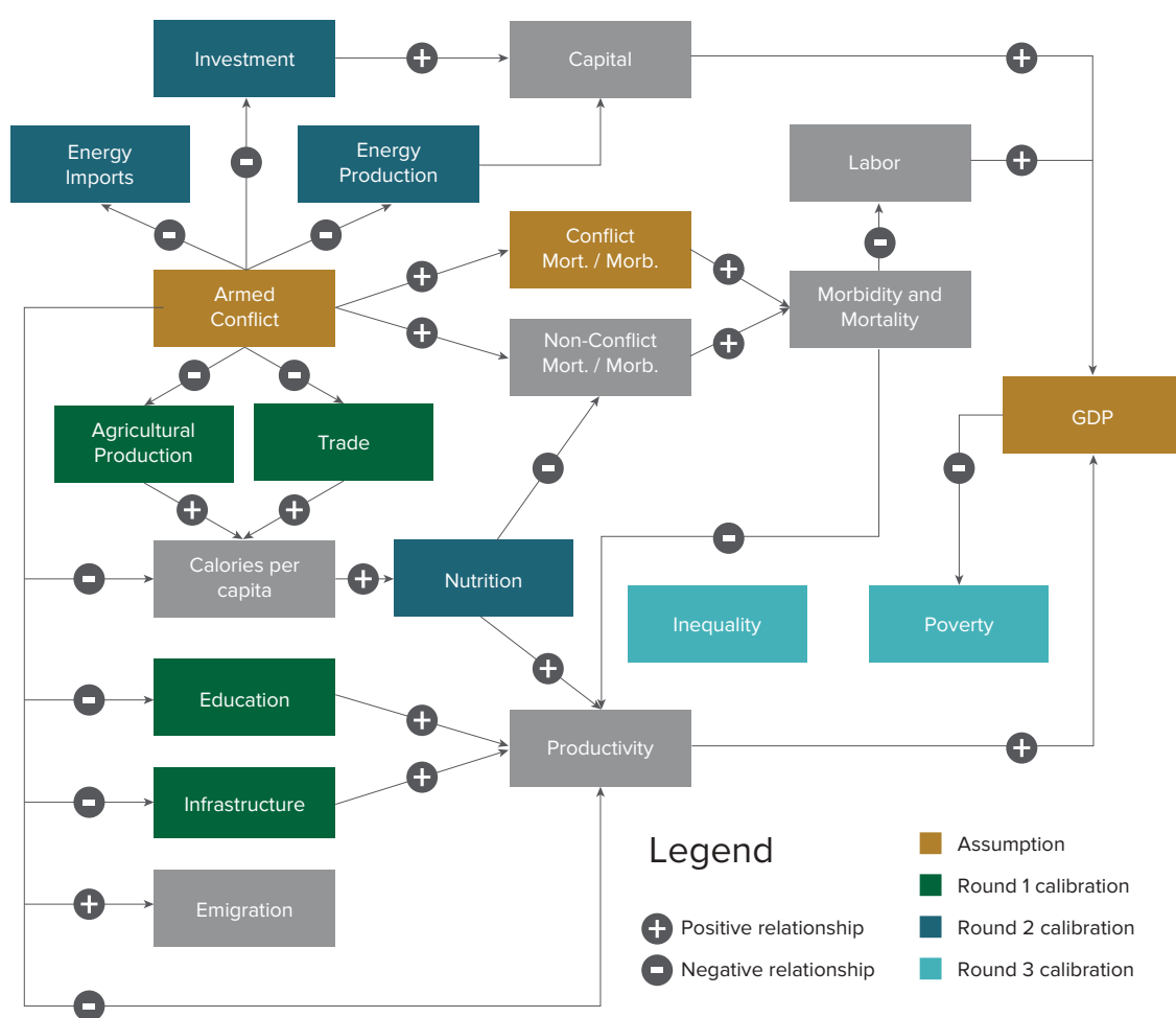
FIGURE 4 | Conceptual model framework used within the International Futures modeling platform.
